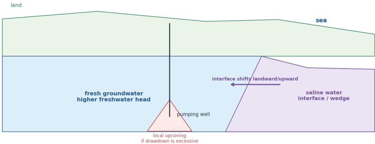
Freshwater head, saline interface and pumping-induced upconing
