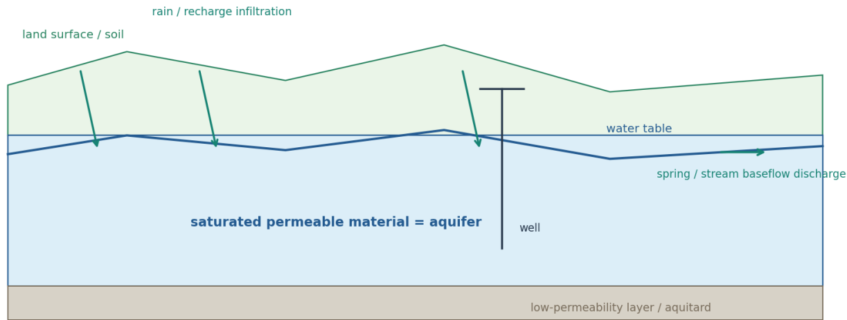
Original deterministic schematic • not to scale • conceptual learning aid Aquifer water budget and cross-section
